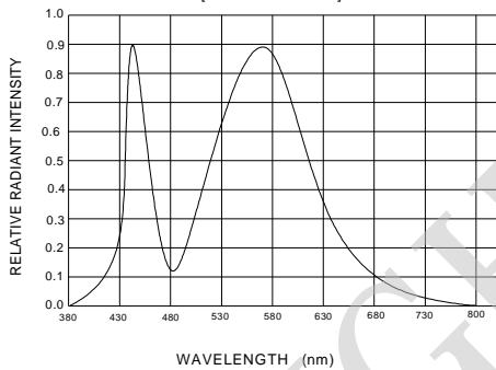
Fig.1 RELATIVE INTENSITY VS. WAVELENGTH [I F =60mA Ta=25±]
