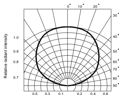
Fig.6 Radiation diagram
