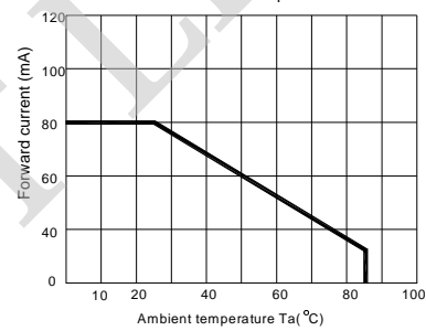
Fig.2 Forward current derating curve vs. ambient temperature
